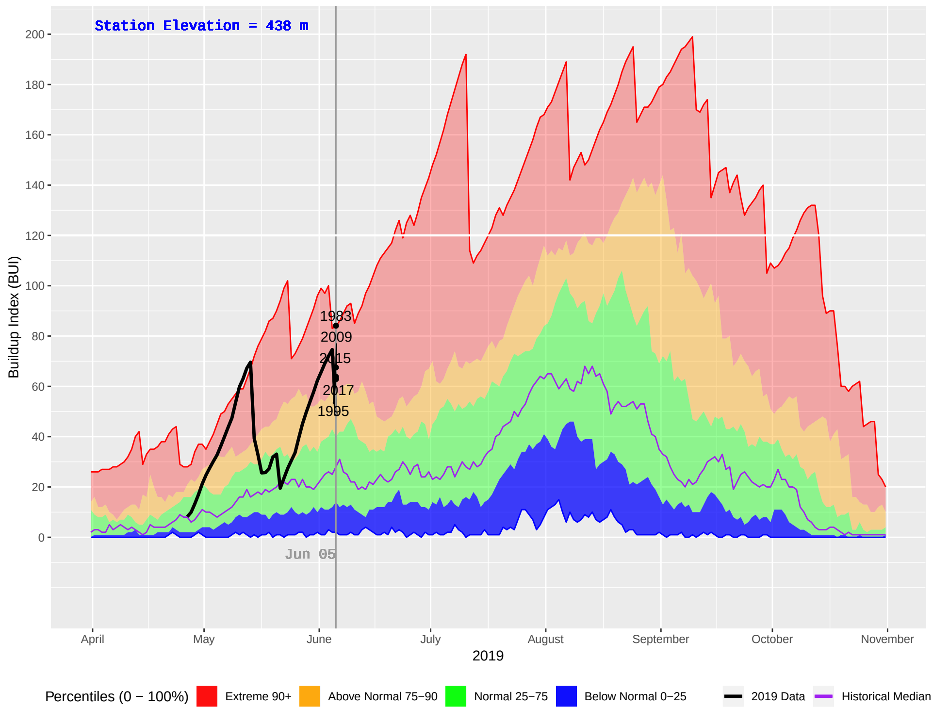
MENZIES CAMP (19) : Historical (1970–2018), Current (2019) Daily Buildup Index (BUI)
