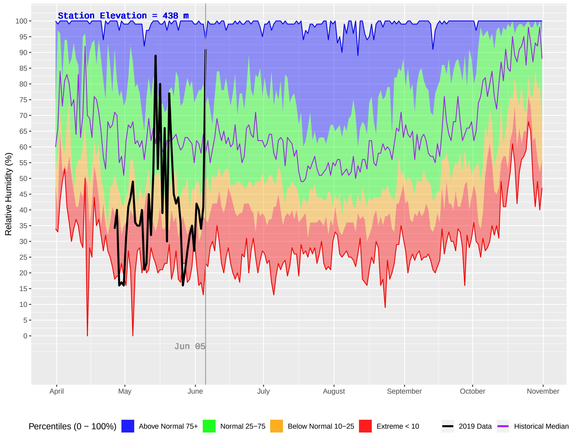
MENZIES CAMP (19) : Historical (1970–2018) and Current (2019) Daily Relative Humidity
