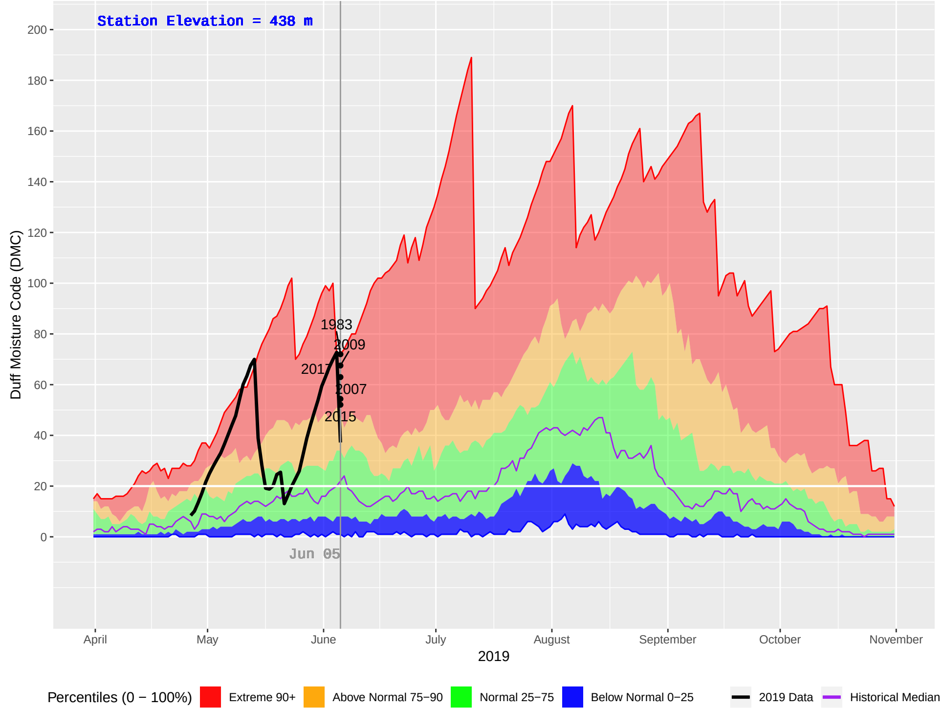
MENZIES CAMP (19) : Historical (1970–2018), Current (2019) Daily Duff Moisture Code (DMC)
