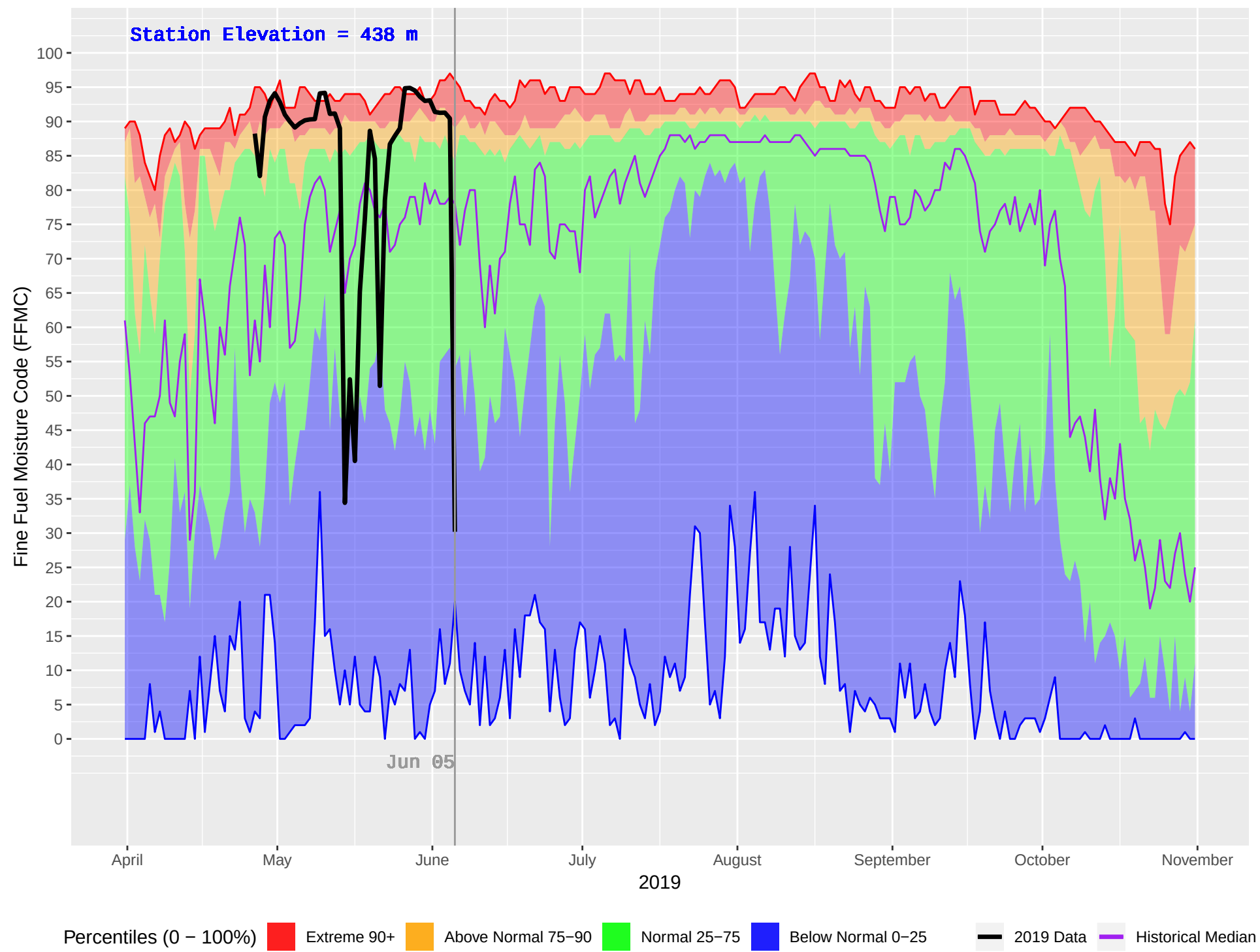
MENZIES CAMP (19) : Historical (1970–2018) and Current (2019) Daily Fine Fuel Moisture Code (FFMC)
