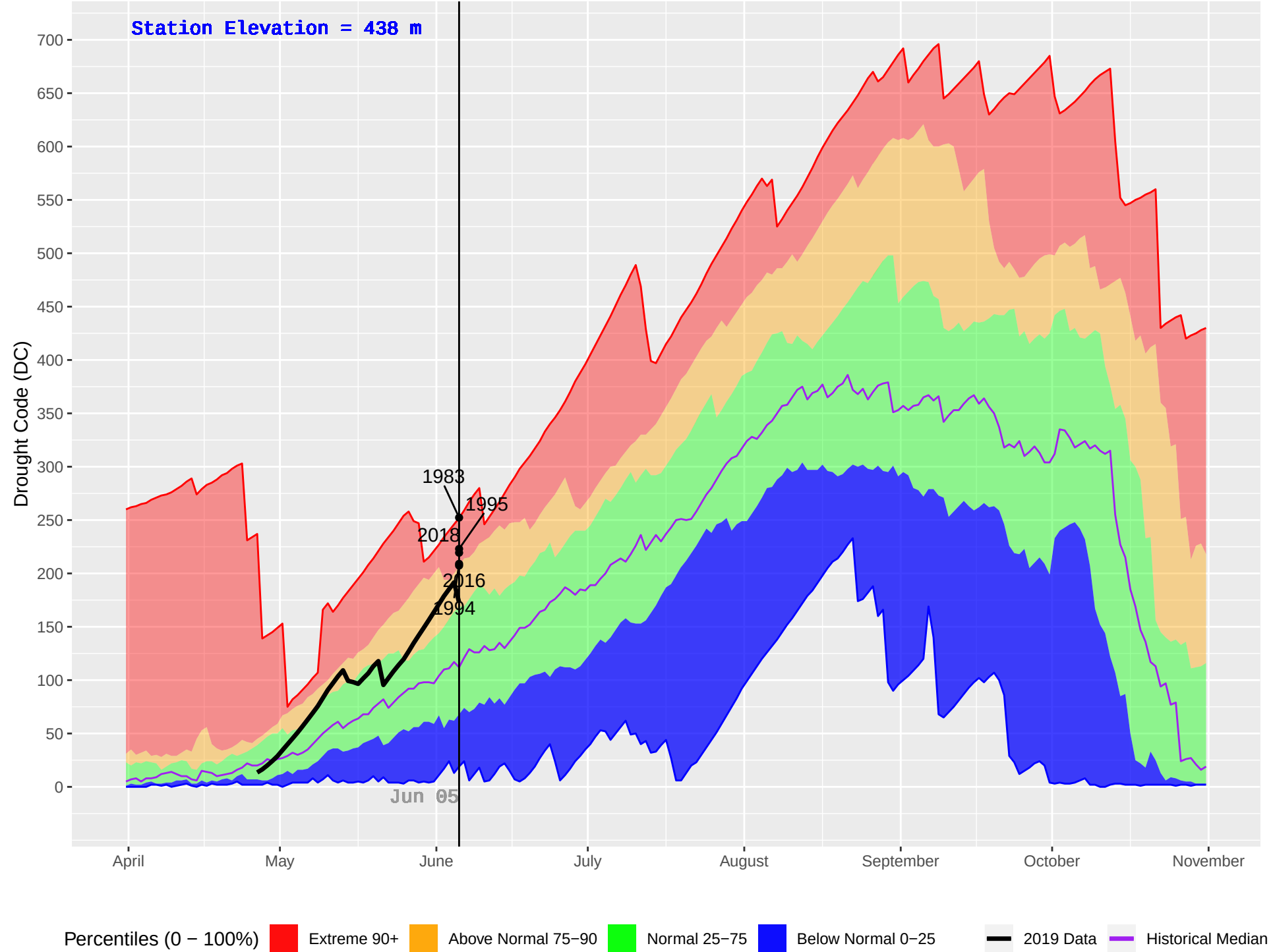
MENZIES CAMP (19) : Historical (1970–2018) and Current (2019) Daily Drought Code (DC)
